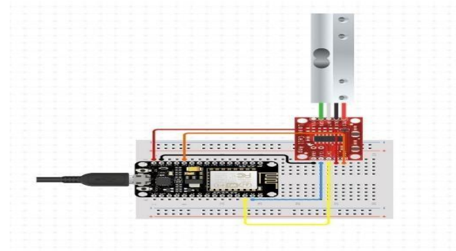
Fig. 5 Hardware circuit connections
