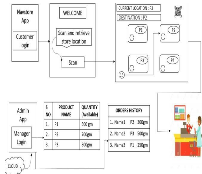
Fig. 4 APP design Overview
