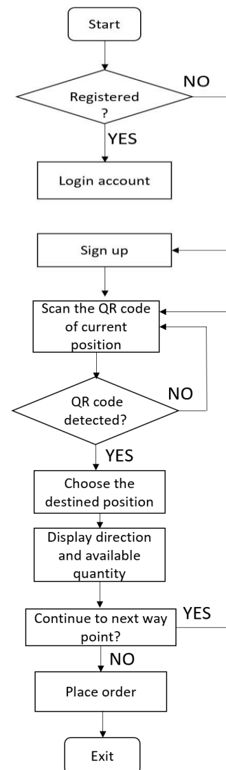
Fig. 2 Flowchart for customer login
