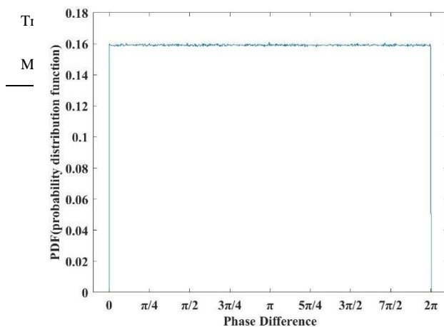
Fig. 6 PD distribution of AWGN channel
